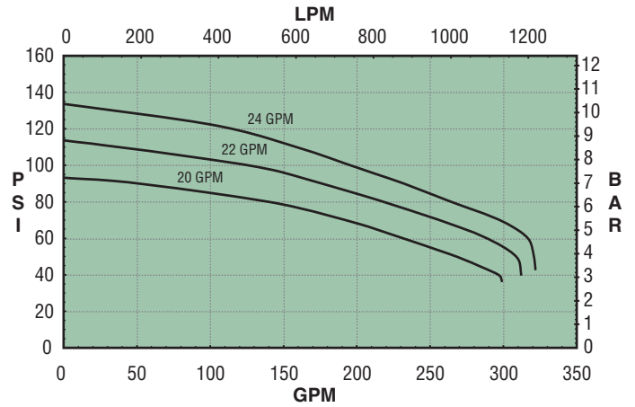
9306C-HM5C-3U & 9306S-HM5C-3U
