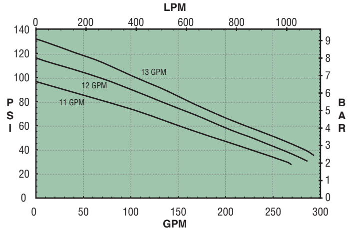
9306C-HM3C-3U & 9306S-HM3C-3U
