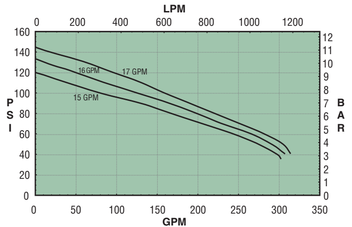
9306C-HM5C-3U & 9306S-HM5C-3U
