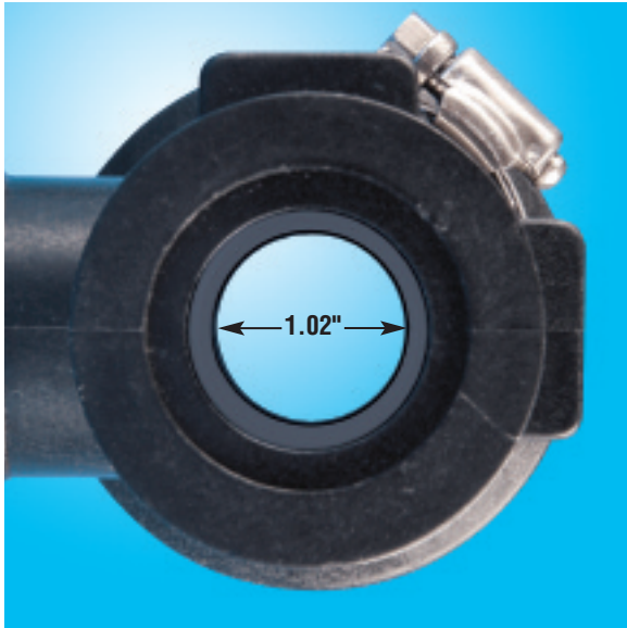
Hypro Universal Gasket (less restrictive)
